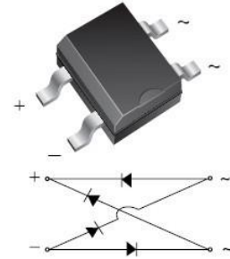
TO-269AA (MBS)
