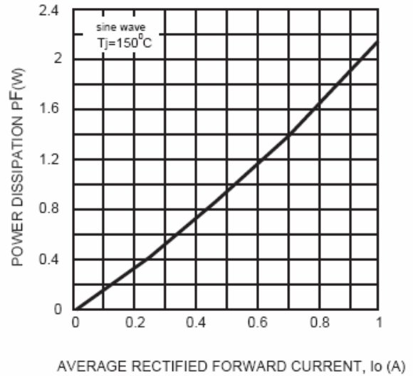
POWER DISSIPATION
