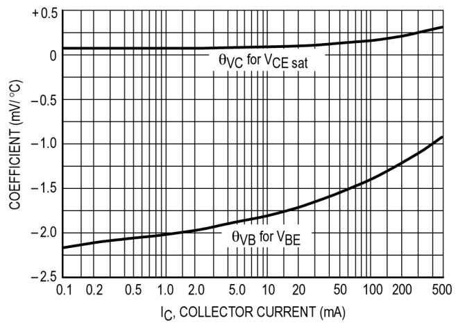
Temperature Coefficients
