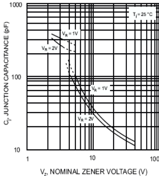
Fig. 4 Junction Capacitance vs Nominal Zener Voltage
