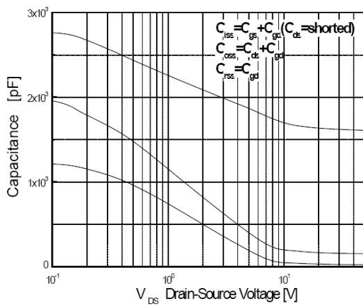
Capacitance Characteristics
