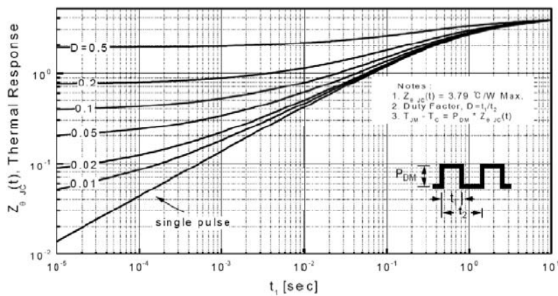
Transient Thermal Response Curve For JCS5N60FB
