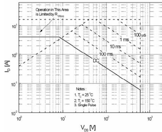
Maximum Safe Operating Area For JCS5N60FB
