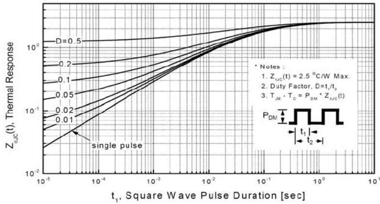
Transient Thermal Response Curve For JCS5N60CB
