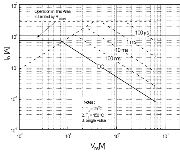
Maximum Safe Operating Area For JCS7N65FB(TO-220MF)
