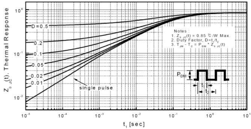
Transient Thermal Response Curve For JCS7N65FB(TO-220MF)
