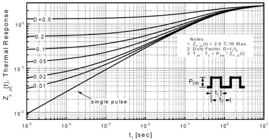
Transient Thermal Response Curve For JCS7N65FB(TO-220MF)
