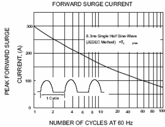
FIG.2-MAXIMUM NON-REPETITIVE PEAK
