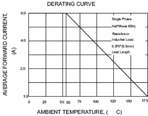
FIG.1-TYPICAL FORWARD CURRENT
