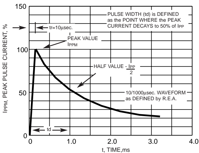
FIG. 3 - PULSE WAVEFORM
