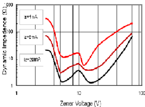
Fig.3 Effect of Zener Voltage on Impedance
