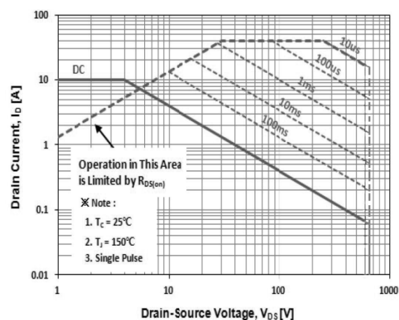
Maximum Safe Operating Area TO-220MF
